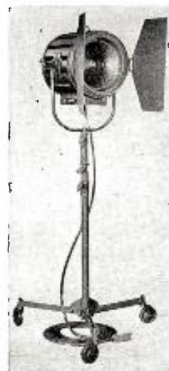
THE BLUE ZEPHYR JUNIOR The finest in modern lighting equipment. Lamp head features include interlocking ventilation channels, direct-action focusing with graduated scale. Attached rotating barn doors and full-size diffuser frame. Stand has folding legs with rubber-tired ball-bearing casters. Adjustable from 51 inches to 113 inches. Blue wrinkle finish.
